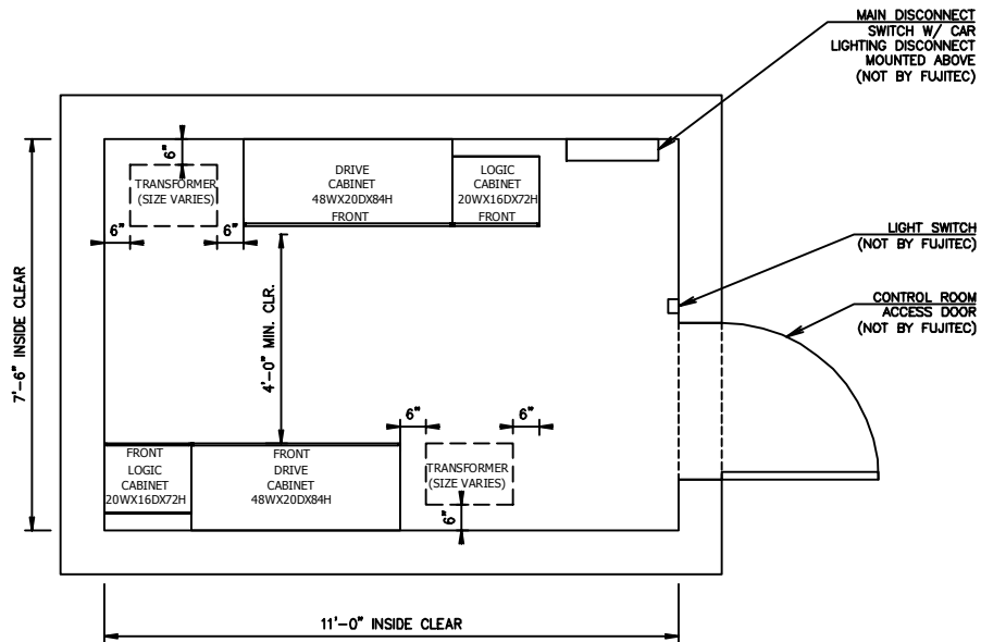
CONTROL ROOM - HVF W/ TRANSFORMER
