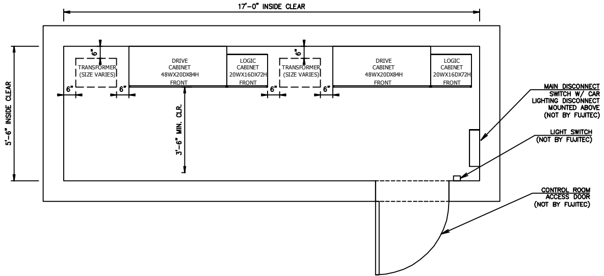
CONTROL ROOM - HVF W/ TRANSFORMER
